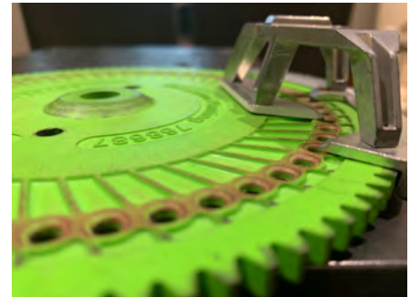
Figure 2. Corn Singulator
